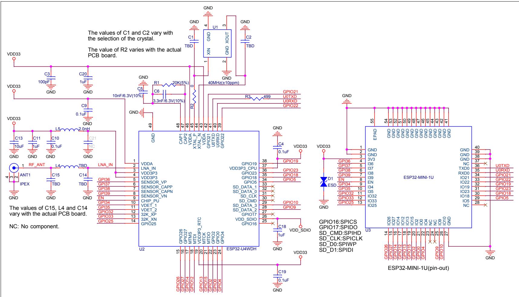
Figure 9: ESP32-MINI-1U Schematics
