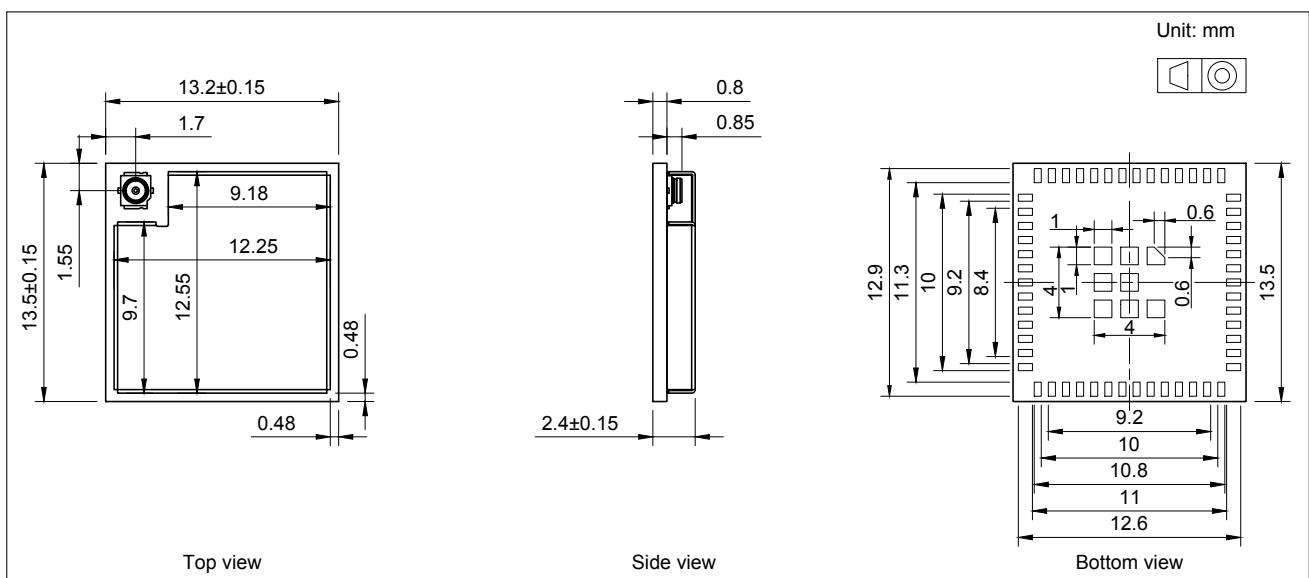
Figure 12: ESP32-MINI-1U Physical Dimensions
