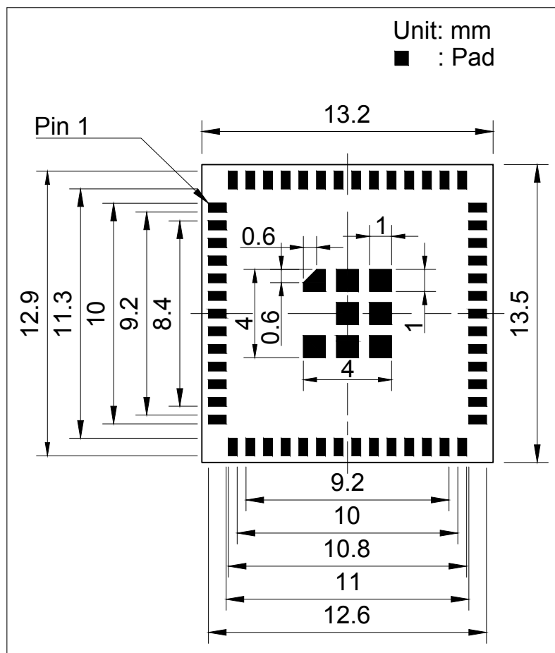
Figure 15: ESP32-MINI-1U PCB Recommended PCB Land Pattern
