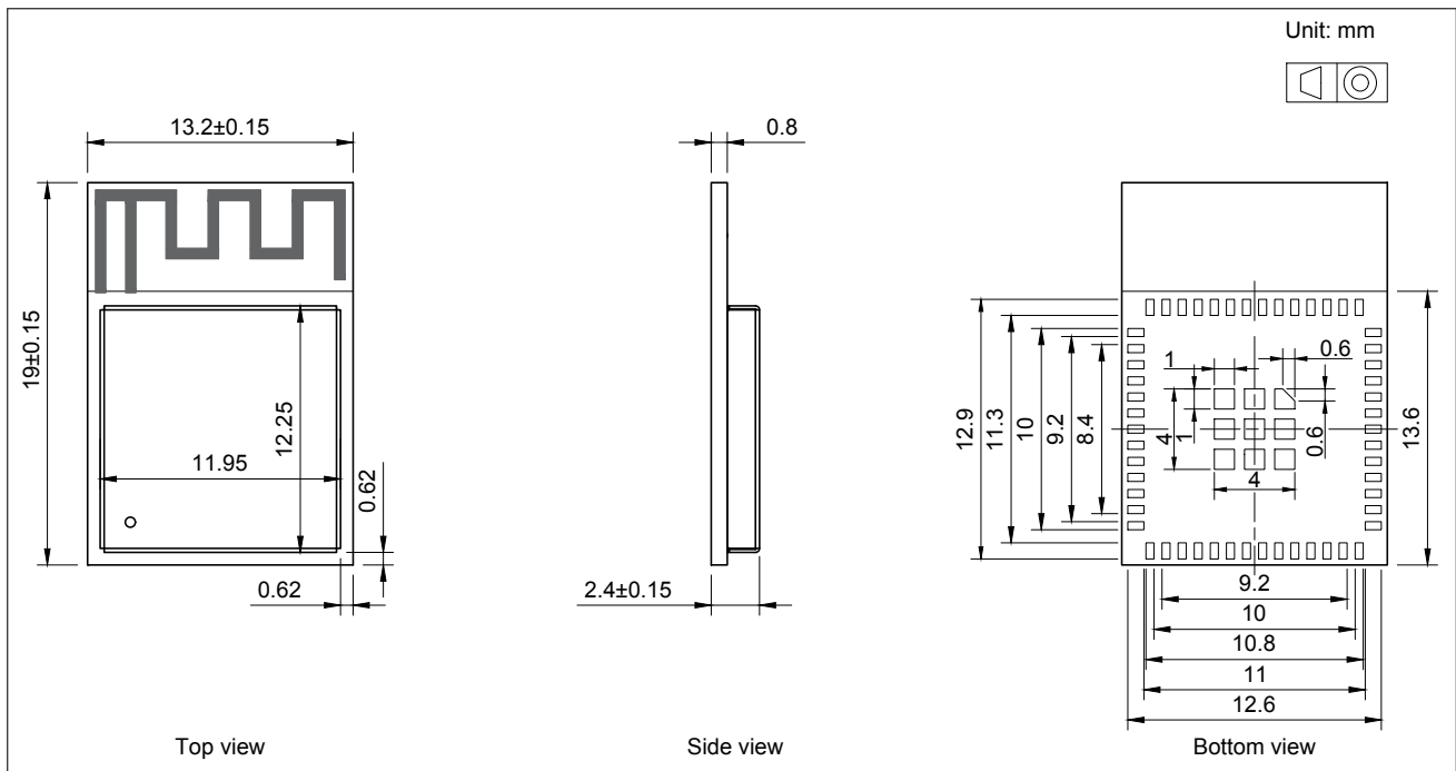
Figure 11: ESP32-MINI-1 Physical Dimensions
