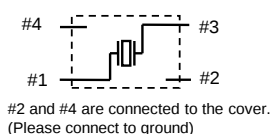
Internal connection (TOP VIEW)
