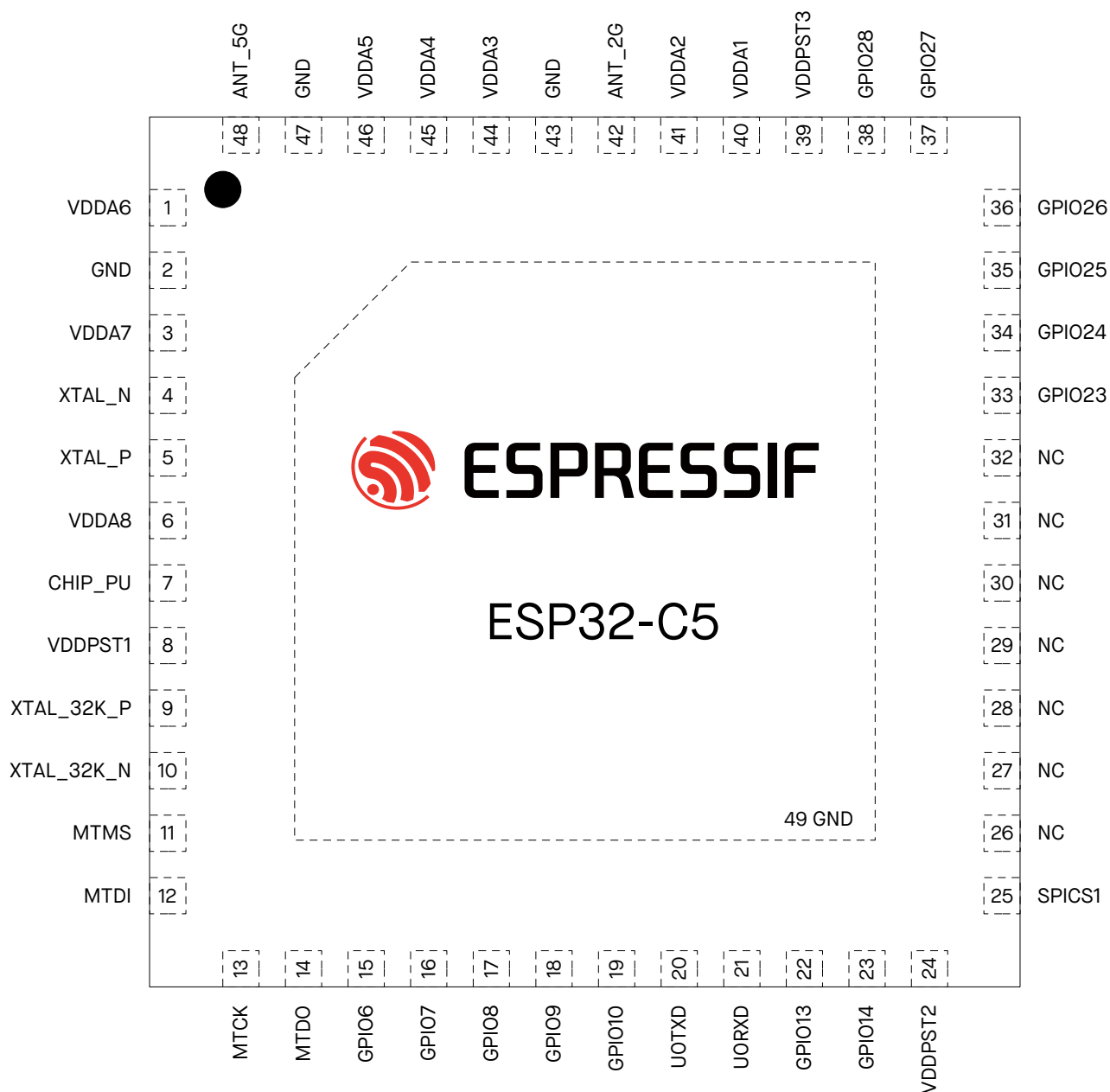
Figure 2-2. ESP32-C5HF4 Pin Layout (Top View)
