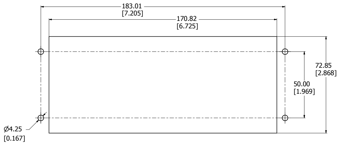
MOUNTING OPENING
