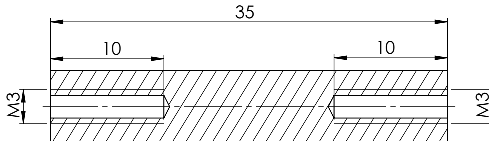
SECTION Y-Y
