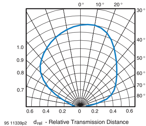
Fig. 12 - Vertical Directivity
